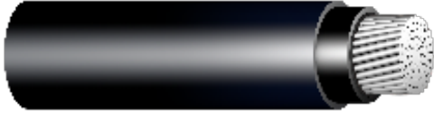
1- Core AL/PVC/Sheathed 600/1000 V Cables as per IEC 60502-1
