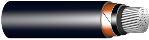
1-Core AL/PVC/CUT/Sheathed 600/1000 V Cables as per IEC 60502-1
